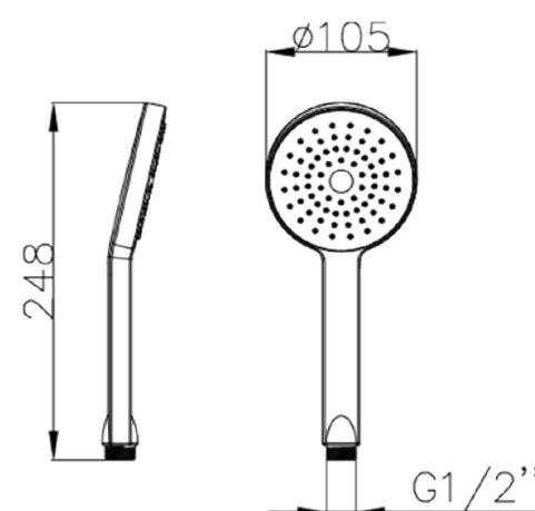
S905/3F 3 Functions: Spray Massage Massage+Spray Φ 105mm
