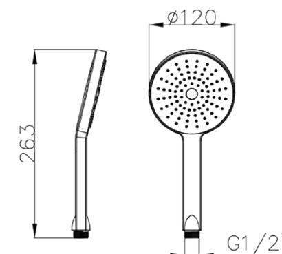
S906/1F 1 Function: Big Spray Φ 120mm
