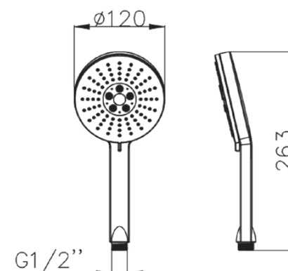
S904/3F 3 Functions: Big Spray Bubbling Bubbling+Spray Φ 120mm
