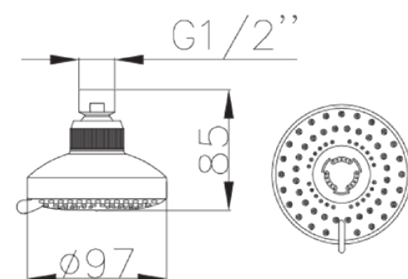
S08/3F 3 Functions: Spray Massage Massage+Spray Ø 97mm
