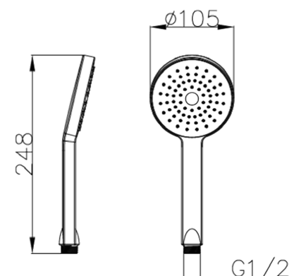
S907/1F 1 Function: Spray Φ 105mm
