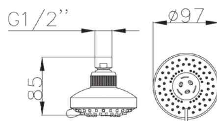
S07/3F 3 Functions: Spray Massage Massage+Spray Ø 97mm
