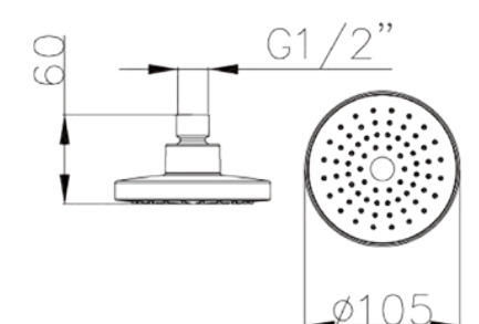
S15/1F 1 Function: Spray Ø 105mm
