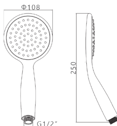
S903/3F 3 Functions: Spray Massage Massage+Spray Φ 108mm
