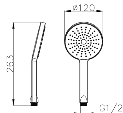
S908/1F 1 Function: Spray Φ 120mm
